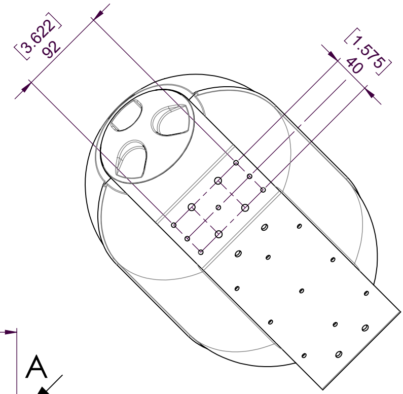
VIEW A
